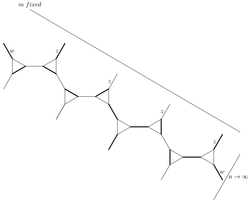
Figure 4.5: Before change of configurations on \mathcal{C}_0
