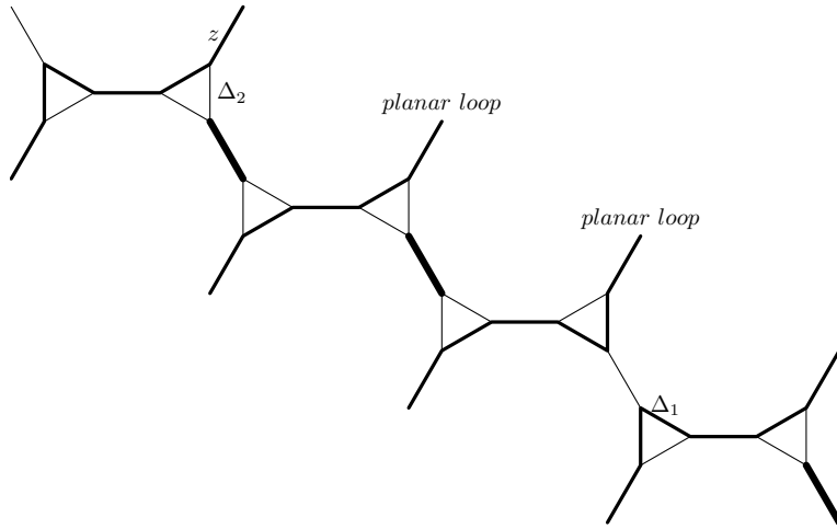
Figure 3.1: before path change
