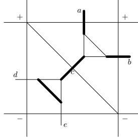
Figure 4.3: Generalized Fisher Correspondence
