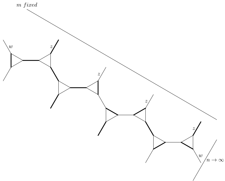
Figure 4.6: After change of configurations on \mathcal{C}_0 to alternating edges
