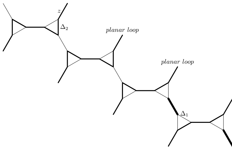
Figure 3.2: after path change
