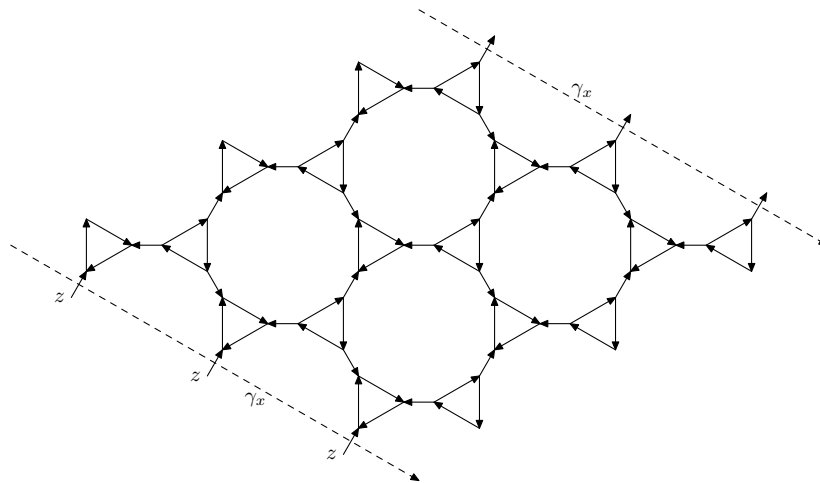
Figure 1.2: Fisher graph on a cylinder
