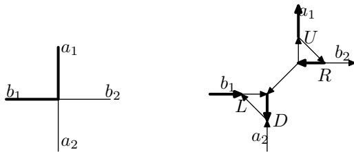
Figure 4.9: vertex of Ising model and corresponding dimer gadget
