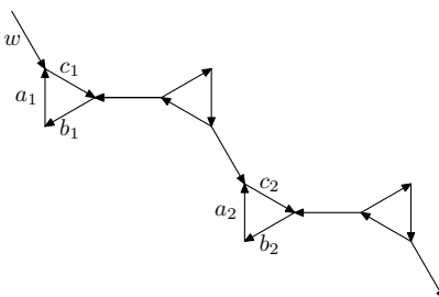
Figure 3.3: 1 \times 2 cylindrical graph
