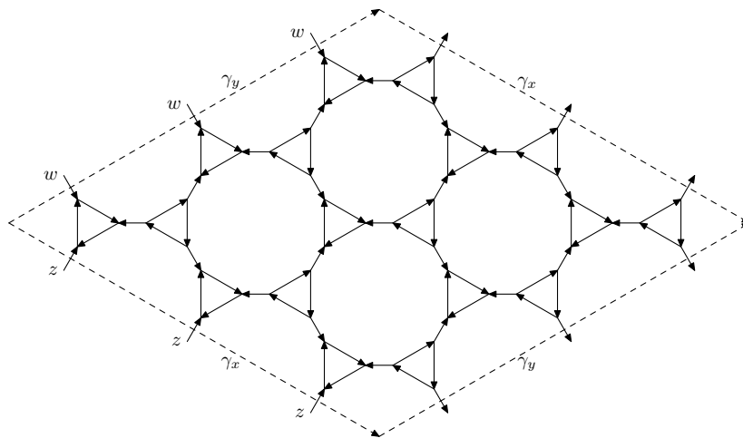
Figure 1.1: Fisher graph
