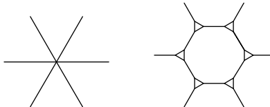
Figure 4.4: Fisher Correspondence
