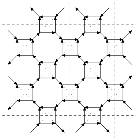
Figure 4.7: Ising model and bipartite graph
