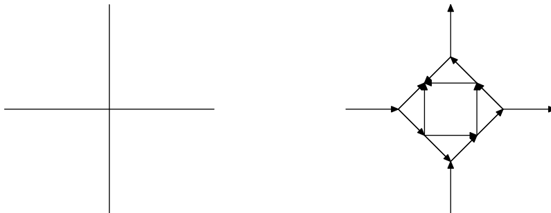
Figure 4.8: Ising model and Fisher graph
