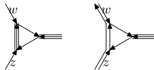
Figure 4.2: local configurations
