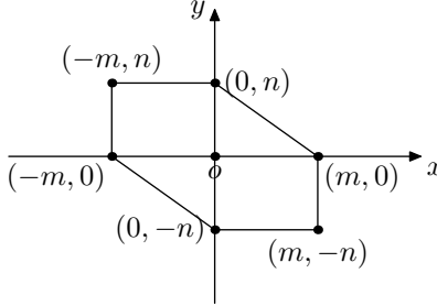
Figure 4.1: Newton polygon
