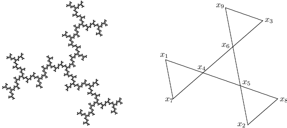
Figure 3. The fractal 3-tree and its V_1 network.
