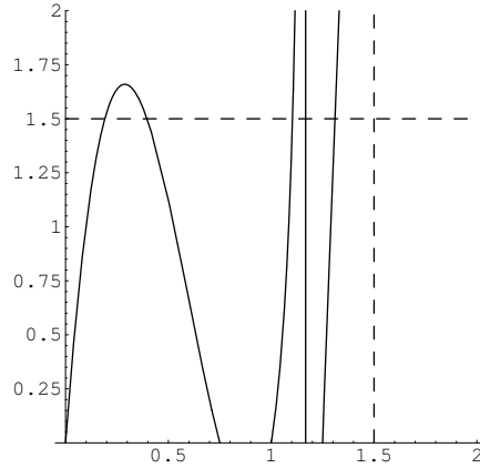
Figure 2. The graph of R(z) for the level-3 Sierpiński gasket.
