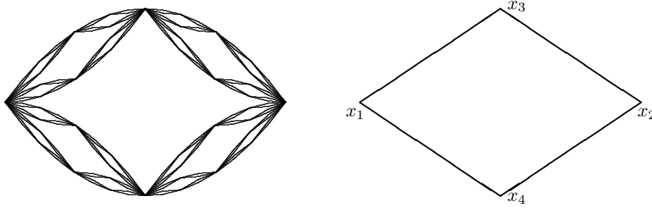
Figure 5. The diamond fractal and its V_1 network.
