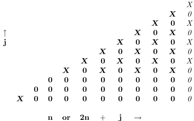
Figure 3: Coefficients of Error Terms
